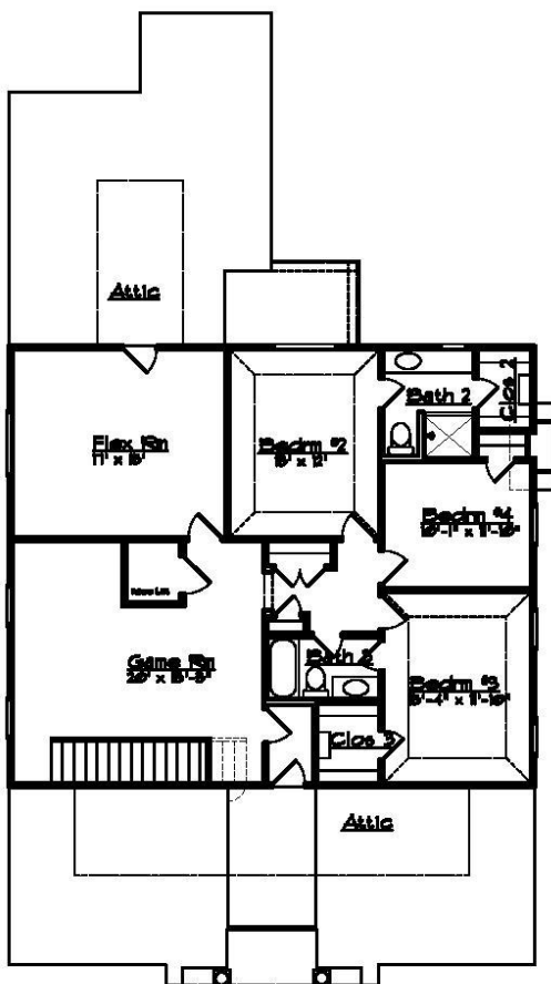
② Second Floor Plan SCALE: NTS
