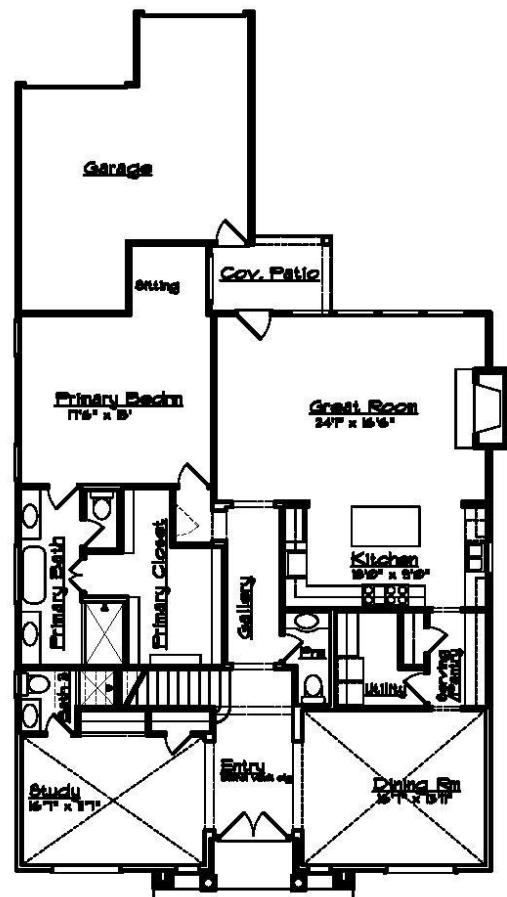
① First Floor Plan SCALE: NTS
